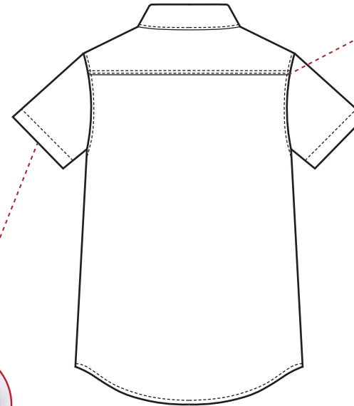
Flat Felled Seam on Armholes & Side Seams
